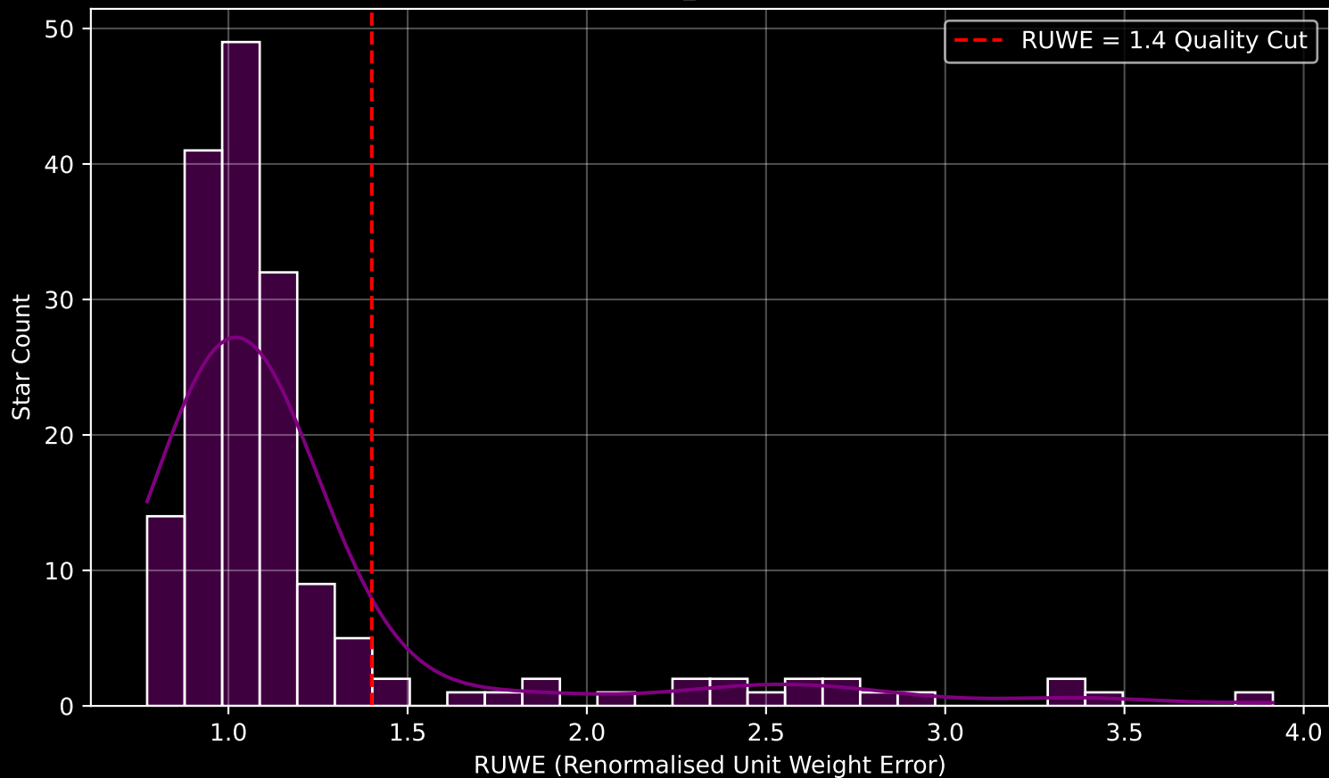
GAPOGEE DR17 Field [085+33_MGA] RUWE Distribution (n= 172)
