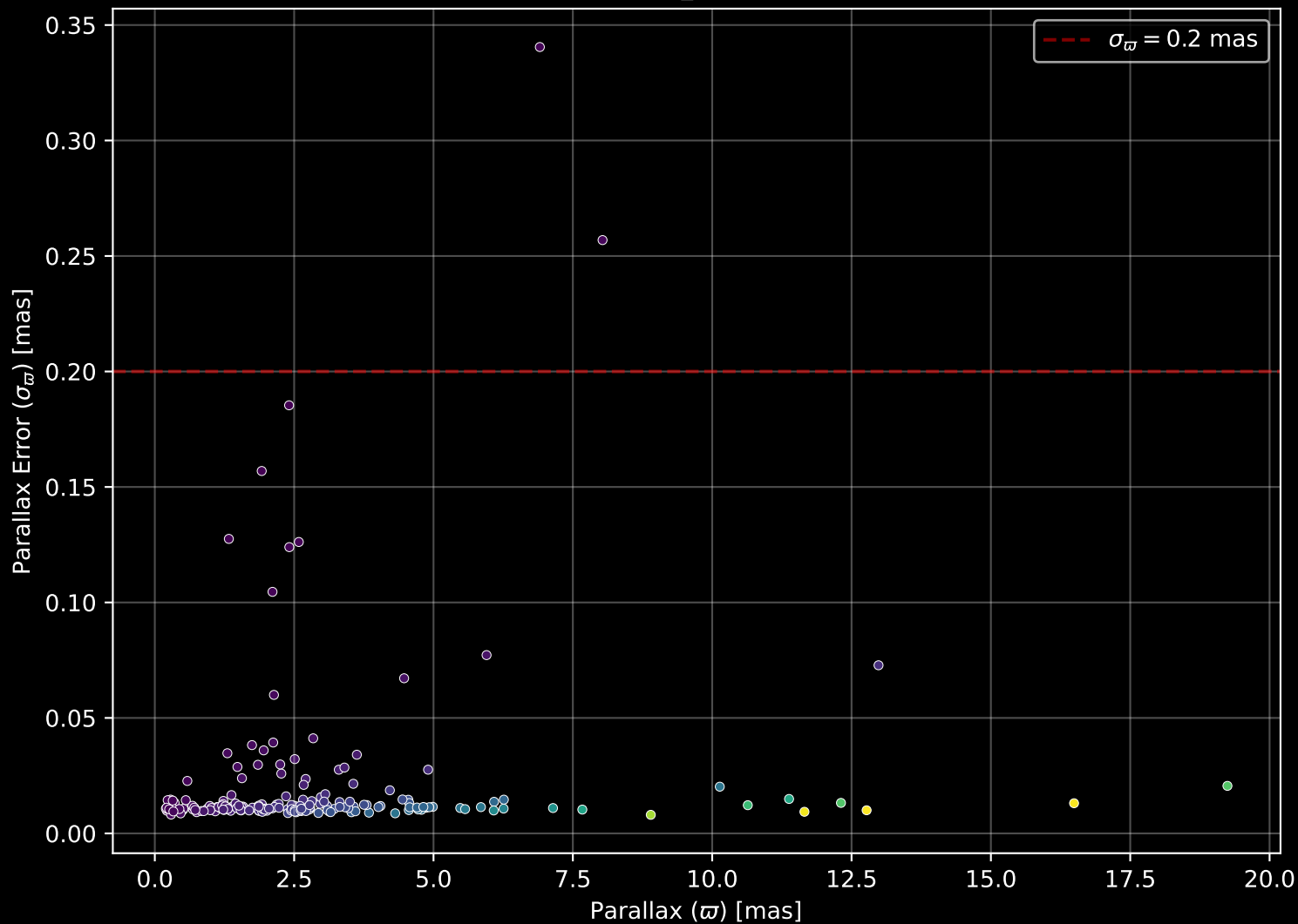
APOGEE DR17 Field: [085+33_MGA] Parallax Quality (n= 184)
