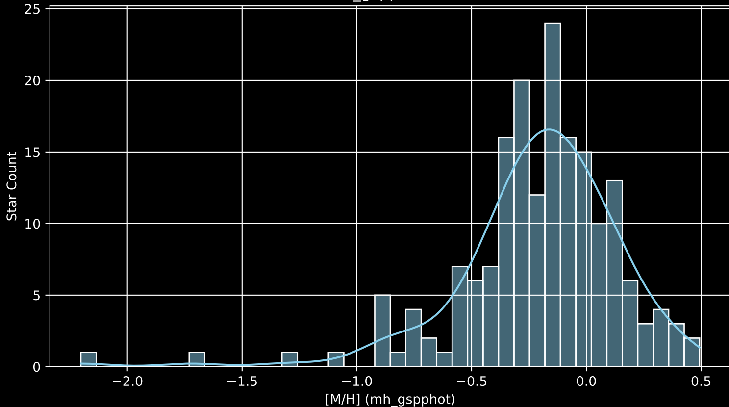
APOGEE DR17 Field: [085+33_MGA [M/H] (mh_gspphot) (n= 181)
