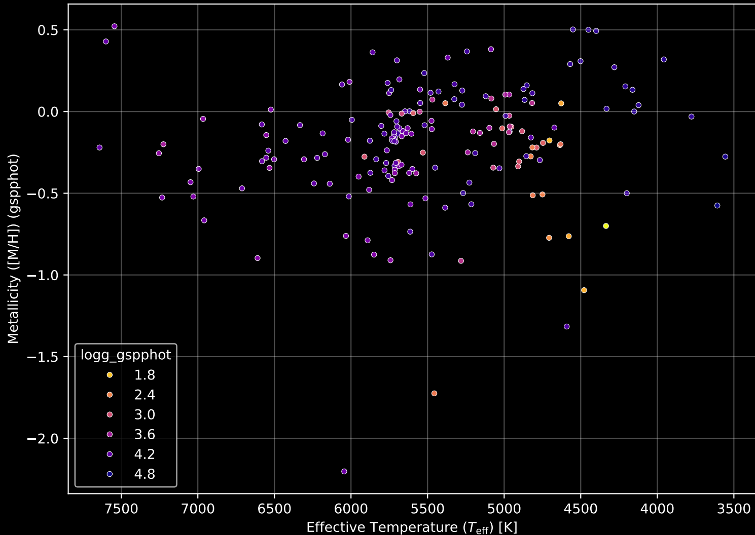
APOGEE DR17 Field: [085+33_MGA] Stellar Population Parameters (n= 184)
