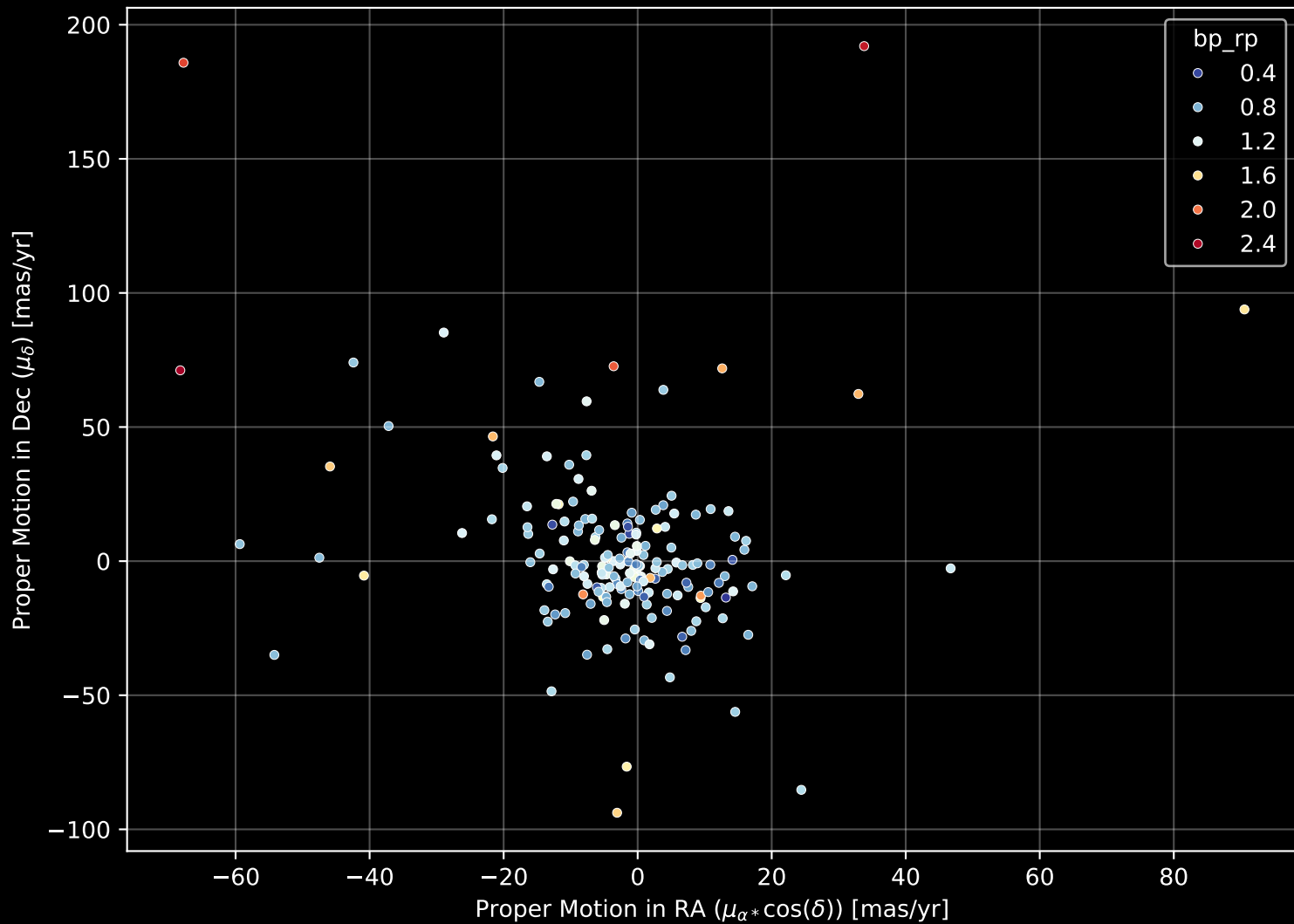
APOGEE DR17 Field: [085+33_MGA] Proper Motion Diagram (n= 184)
