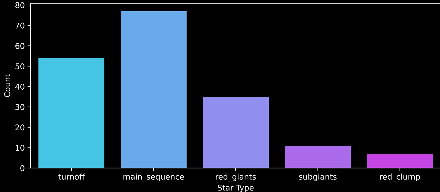
APOGEE DR17 Field: [085+33_MGA] Count plot of Star Type
